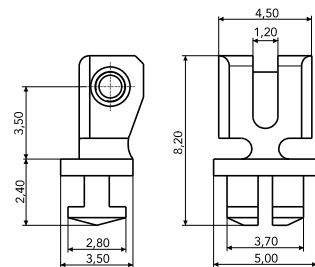
90° INSERT HINGE 03FRA0262A1BN0
