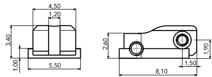
180° FRONT HINGE 03FRA0167A1BN0
