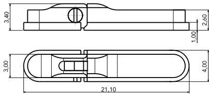
ASSEMBLED HINGE 03ELA0165A1BN0
