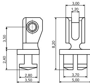
90° INSERT HINGE 03FRA0261A1BN0
