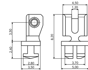
90° INSERT HINGE 03FRA0262A1BN0
