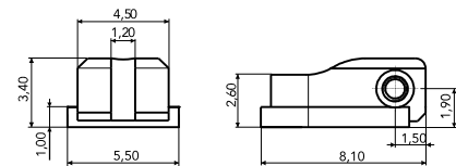
180° FRONT HINGE 03FRA0171A1BN0
