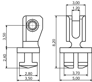
90° INSERT HINGE 03FRA0261A1BN0
