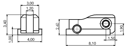
180° FRONT HINGE 03FRA0131A1BN0
