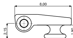
180° INSERT HINGE 03FRC4146A2BN0
