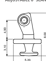
90° INSERT HINGE 03FRC4141A2BN0
