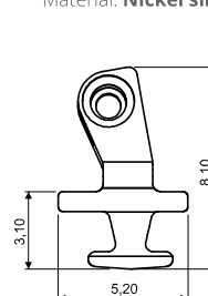
90° INSERT HINGE 03FRC4142A2BN0
