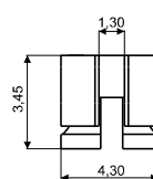
180° INSERT HINGE 03FRC4146A2BN0
