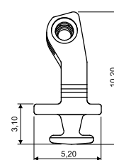
90° INSERT HINGE 03FRC4159A2BN0
