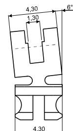
90° INSERT HINGE 03FRC4142A2BN0
