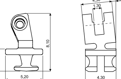
90° INSERT HINGE 03FRC4142A2BN0 Material: Nickel silver ADJUSTABLE 6° SLANTED ANGLE
