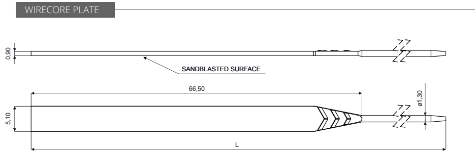
WIRECORE PLATE CODE C4164 Material: Nickel silver
