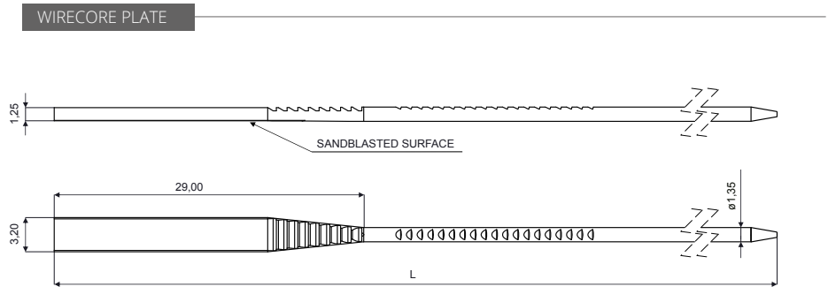
WIRECORE PLATE CODE C7795 Material: Nickel silver
