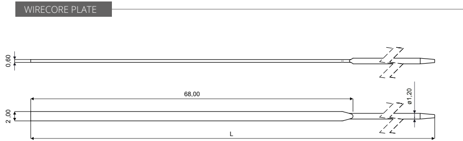
WIRECORE PLATE CODE 20189 Material: Stainless steel
