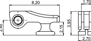
180° INSERT HINGE 03FR27223000 Material: Nickel silver
