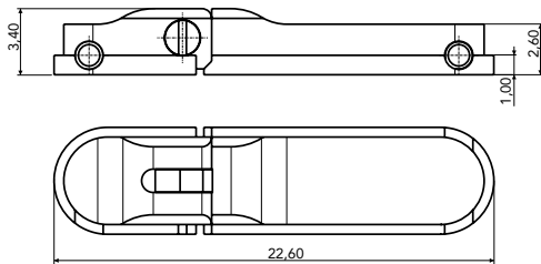
ASSEMBLED HINGE 03ELA0169A1BN0
