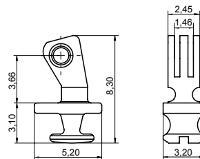
90° INSERT HINGE 03FRC9418A2BN0 Material: Nickel silver ADJUSTABLE
