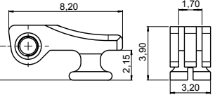
180° INSERT HINGE 03FR32223000 Material: Nickel silver
