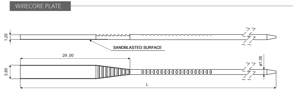
WIRECORE PLATE CODE C7793 Material: Nickel silver
