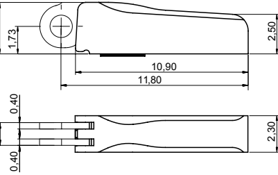
BOX 03SCCB032A1BYX Material: Nickel silver WITH SOLDERING PATCH
