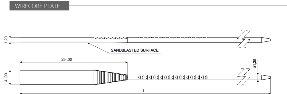
WIRECORE PLATE CODE C7791 Material: Nickel silver
