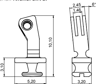
90° INSERT HINGE 03FRC9421A2BN0 Material: Nickel silver HIGH VERSION ADJUSTABLE 6° SLANTED ANGLE
