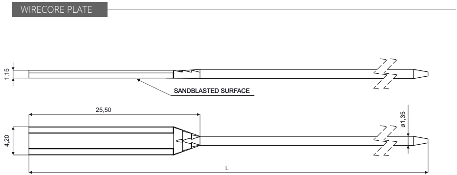
WIRECORE PLATE CODE RET2333 Material: Nickel silver
