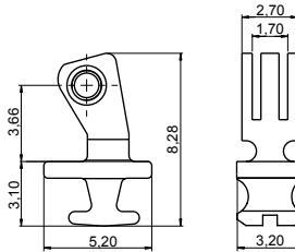
90° INSERT HINGE 03FRC5911A2BN0 Material: Nickel silver ADJUSTABLE
