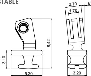
90° INSERT HINGE 03FRC5912A2BN0 Material: Nickel silver ADJUSTABLE 6° SLANTED ANGLE
