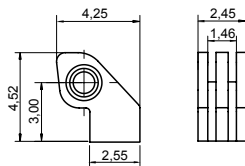
STEP HINGE 03FRC9416A1BY0 Material: Nickel silver
