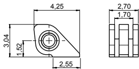
SOLDERING HINGE 03FR27220000 Material: Nickel silver
