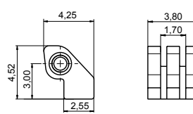
STEP HINGE 03FR38221000 Material: Nickel silver
