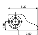
SOLDERING HINGE 03FRC4551A1BY0 Material: Nickel silver
