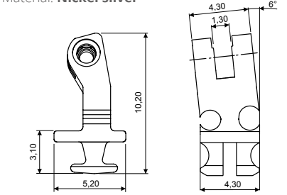
90° INSERT HINGE 03FRC4159A2BN0 Material: Nickel silver HIGH VERSION ADJUSTABLE 6° SLANTED ANGLE
