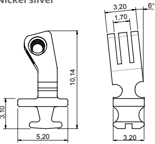
90° INSERT HINGE 03FRC5908A2BN0 Material: Nickel silver HIGH VERSION ADJUSTABLE 6° SLANTED ANGLE
