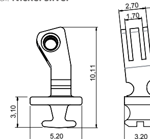
90° INSERT HINGE 03FRC5906A2BN0 Material: Nickel silver HIGH VERSION ADJUSTABLE 6° SLANTED ANGLE
