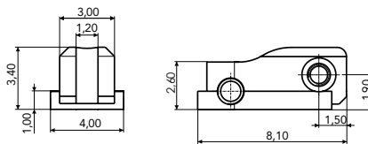
180° FRONT HINGE 03FRA0131A1BN0
