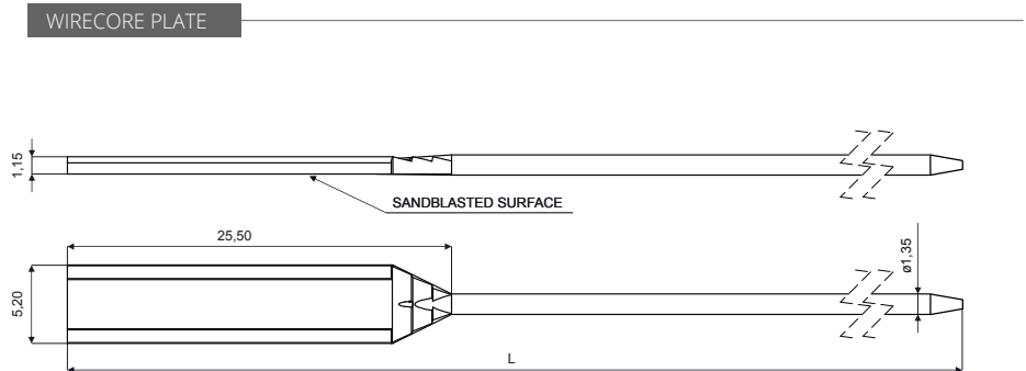
WIRECORE PLATE CODE C8914 Material: Nickel silver
