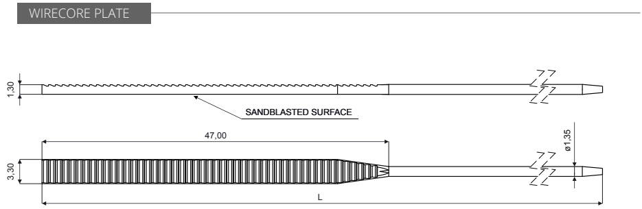
WIRECORE PLATE CODE C1395 Material: Nickel silver
