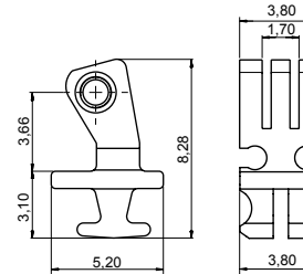
90° INSERT HINGE 03FRC5915A2BN0 Material: Nickel silver ADJUSTABLE
