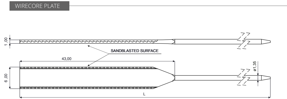
WIRECORE PLATE CODE C7629 Material: Nickel silver
