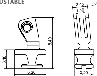
90° INSERT HINGE 03FRC9419A2BN0 Material: Nickel silver ADJUSTABLE 6° SLANTED ANGLE
