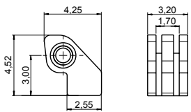
STEP HINGE 03FR32221000 Material: Nickel silver
