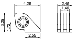
SOLDERING HINGE 03FRC9415A1BY0 Material: Nickel silver
