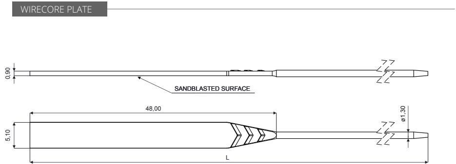
WIRECORE PLATE CODE C1499 Material: Nickel silver
