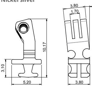
90° INSERT HINGE 03FRC5910A2BN0 Material: Nickel silver HIGH VERSION ADJUSTABLE 6° SLANTED ANGLE
