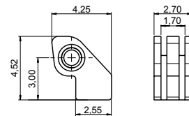
STEP HINGE 03FR27221000 Material: Nickel silver
