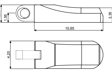
BOX 03SCC4132A1BYX Material: Nickel silver
