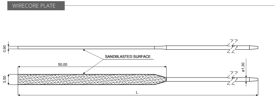
WIRECORE PLATE CODE B0154 Material: Nickel silver
