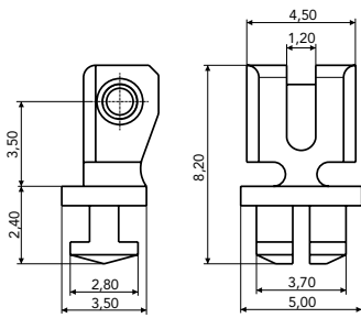
90° INSERT HINGE 03FRA0262A1BN0
