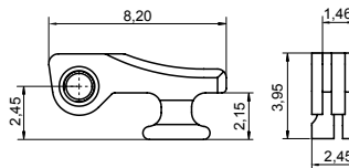
180° INSERT HINGE 03FRC9417A2BN0 Material: Nickel silver
