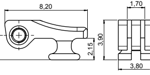
180° INSERT HINGE 03FR38223000 Material: Nickel silver
