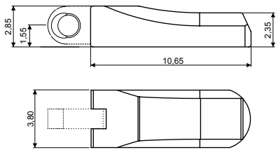
BOX 03SCC4131A1BYX Material: Nickel silver
